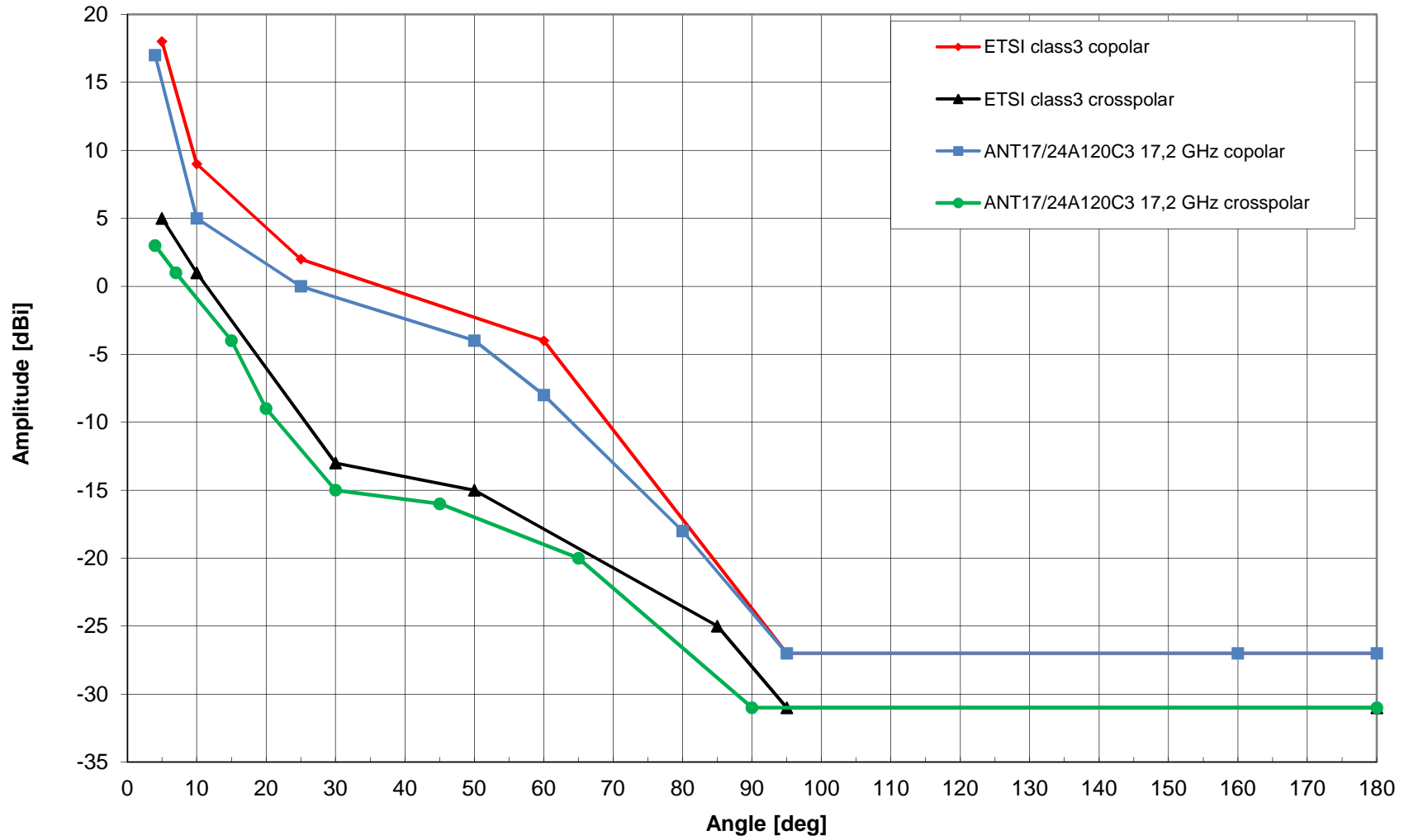
Radiation pattern ANT17/24A120C3 17,2 GHz, max. gain 43,0 dBi
