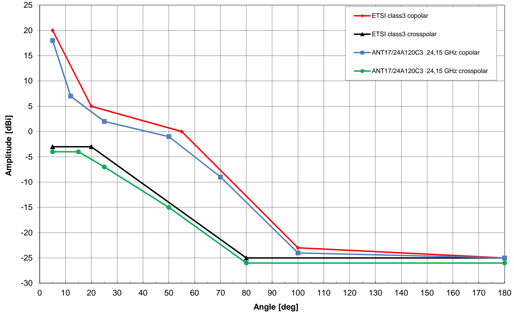
Radiation pattern ANT17/24A120C3 24,15 GHz, max. gain 45,5 dBi
