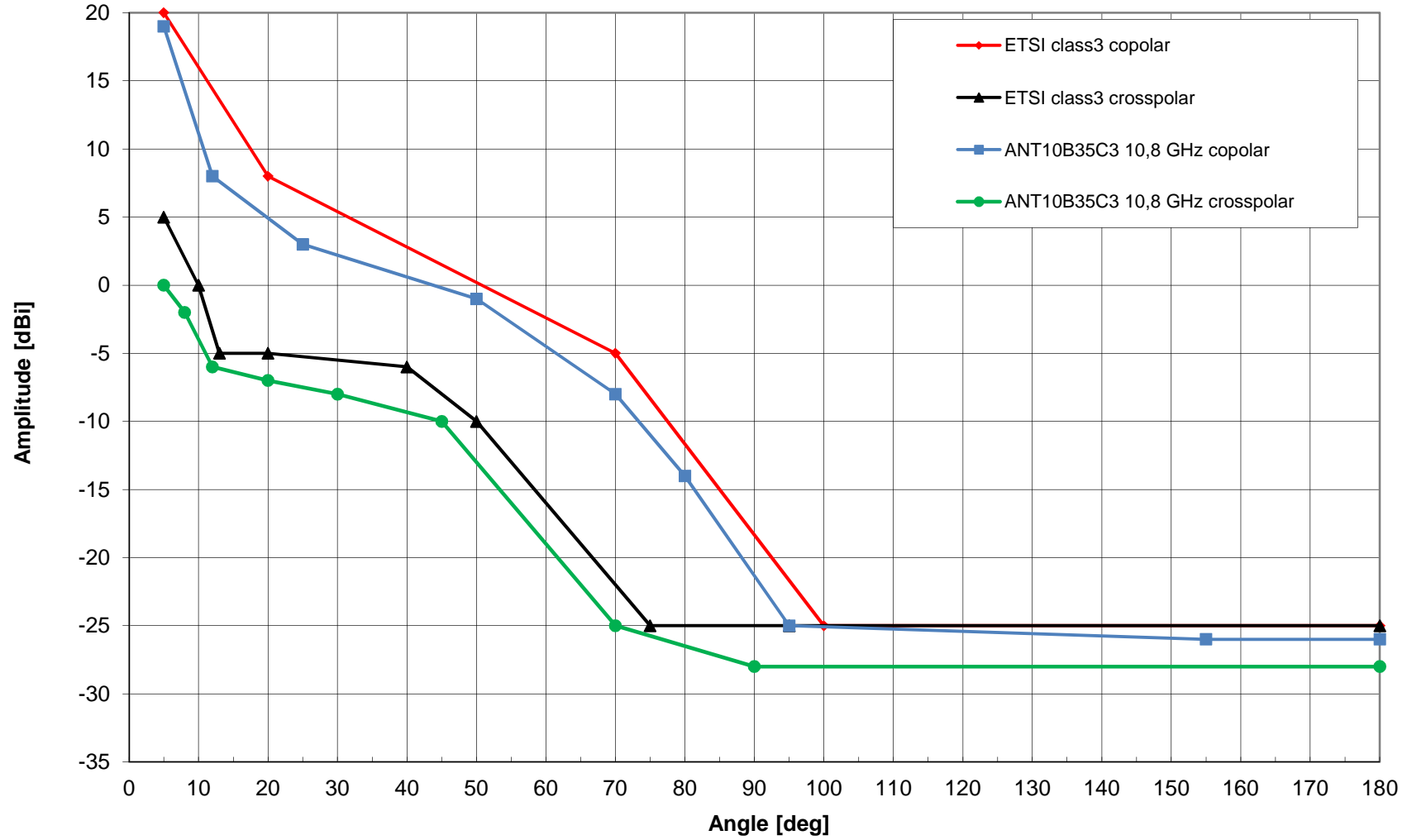
Radiation pattern ANT10B35C3 10,8 GHz, max. gain 29,4 dBi
